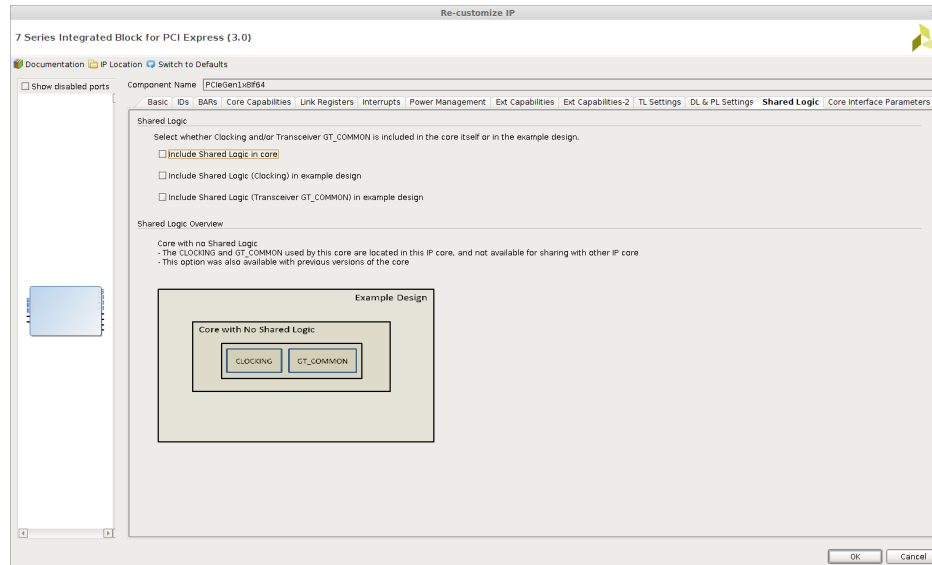
Figure 4.9: Shared Logic Tab
