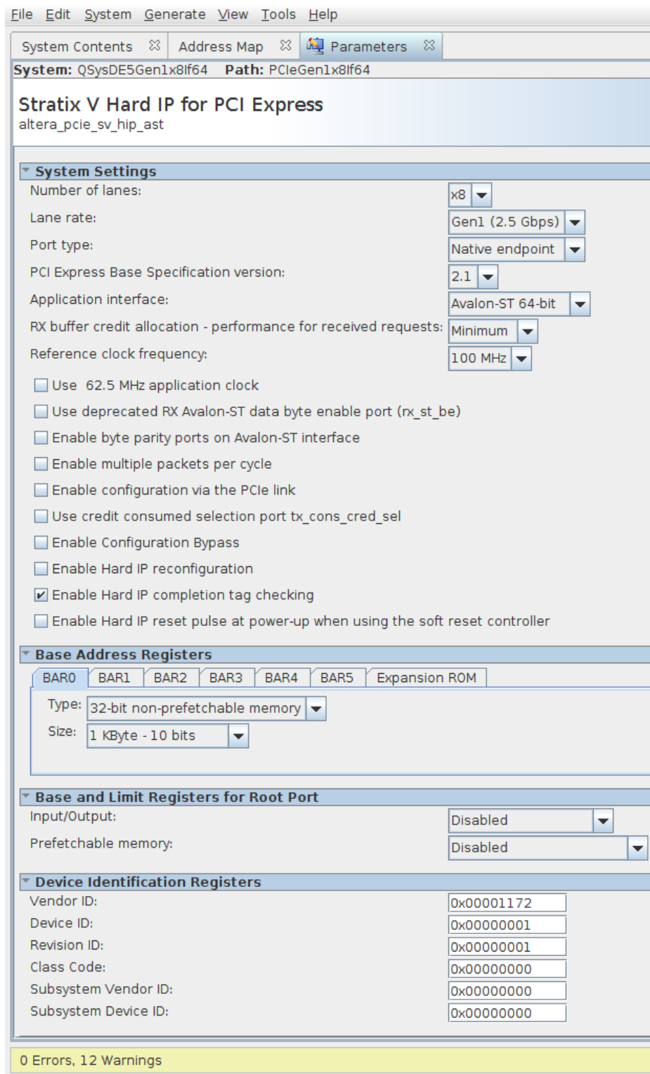
Figure 5.5: PCI Express Endpoint Configuration Menu
