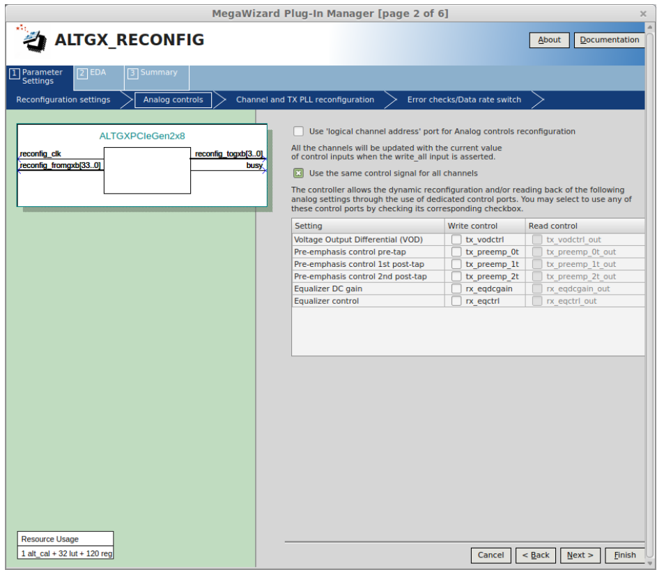
Figure 5.16: ALTGX Reconfiguration Analog Settings Tab
